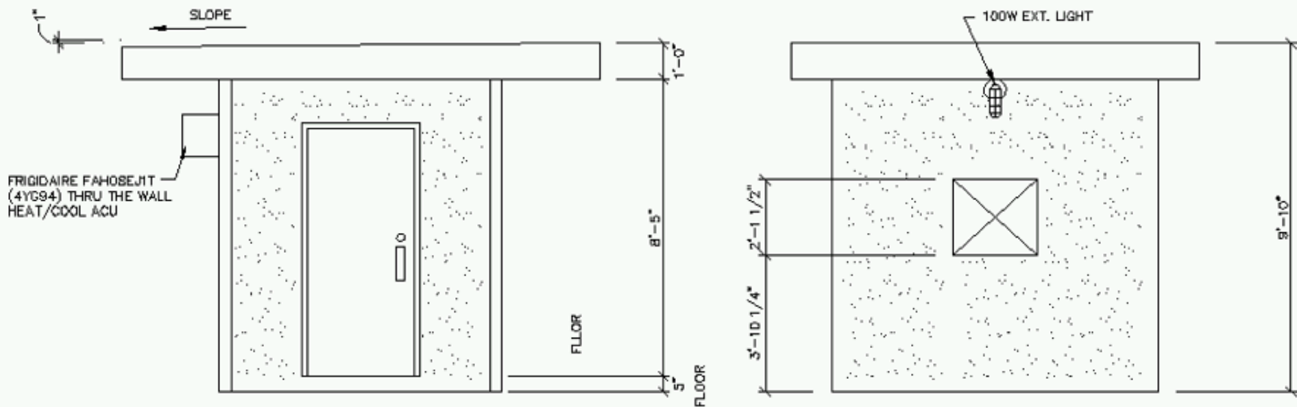
LEFT ELEVATION
